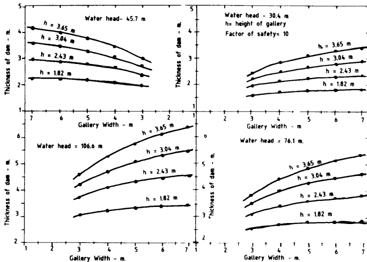
FIG. 2. DAM THICKNESS FOR VARIOUS HYDROSTATIC HEADS, GALLERY WIDTH AND HEIGHTS AS PER THICK PLATE EQUATION-11
