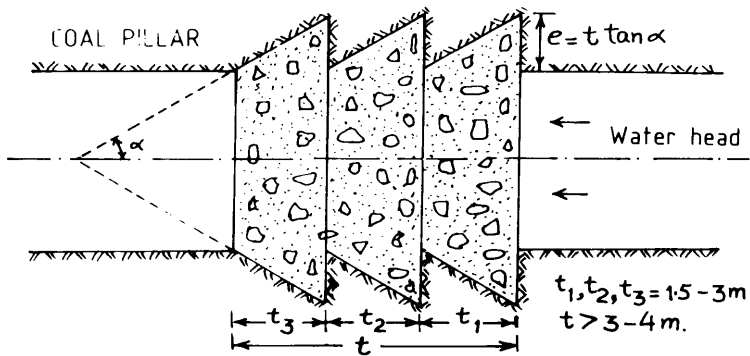
FIG. 4. A MULTY-STAGE WATER DAM.
