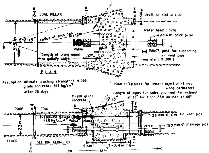
FIG. 3. CONSTRUCTIONAL DETAILS OF AN UNDERGROUND WATER DAM
