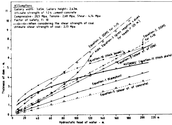
FIG-1. THICKNESS OF DAM AGAINST HYDROSTATIC HEAD- COMPARISON OF VARIOUS APPROACHES.
